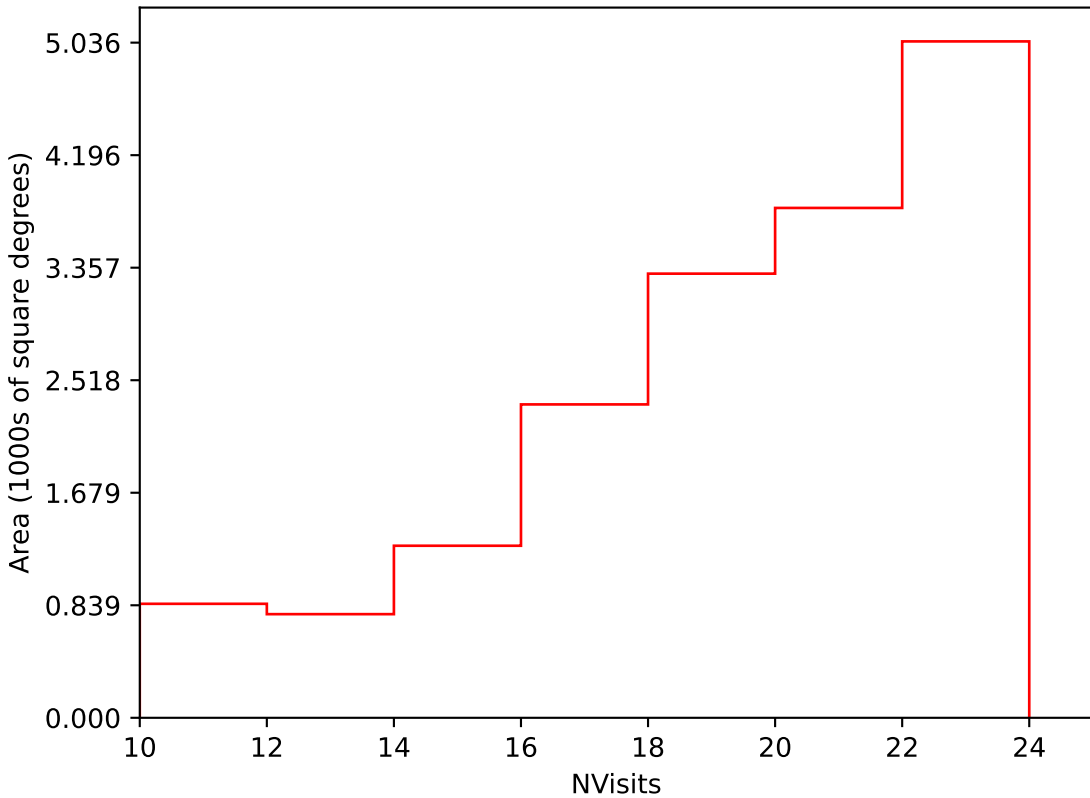
weather_cloudso4v3.4_10yrs Yr 1 i band: NVisits
