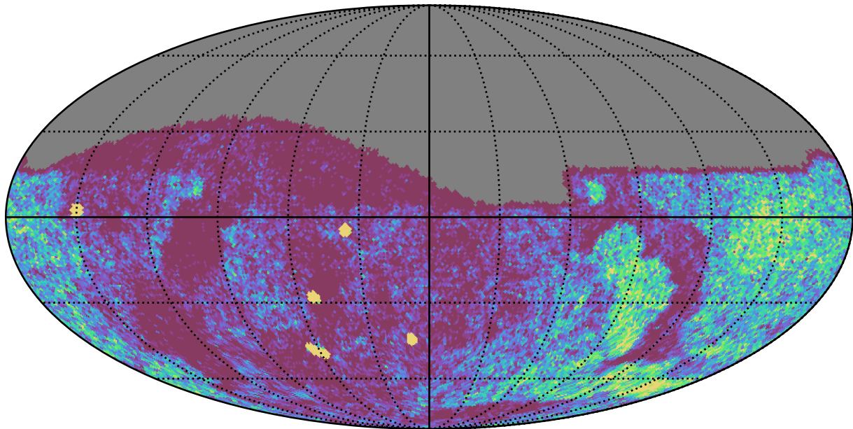
weather_cloudso4v3.4_10yrs Yr 1 g band: NVisits
