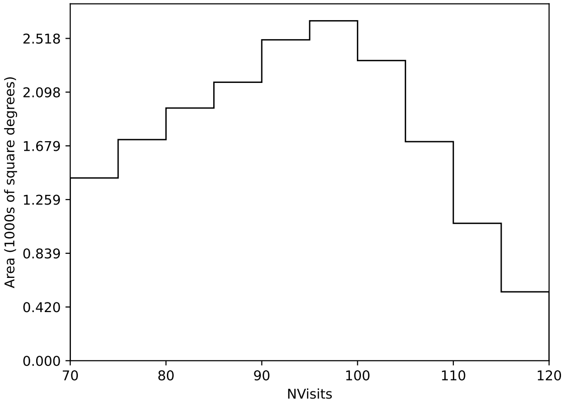
weather_cloudso4v3.4_10yrs Yr 1 all bands: NVisits
