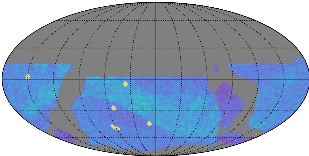
weather_cloudso4v3.4_10yrs WFD z band: NVisits
