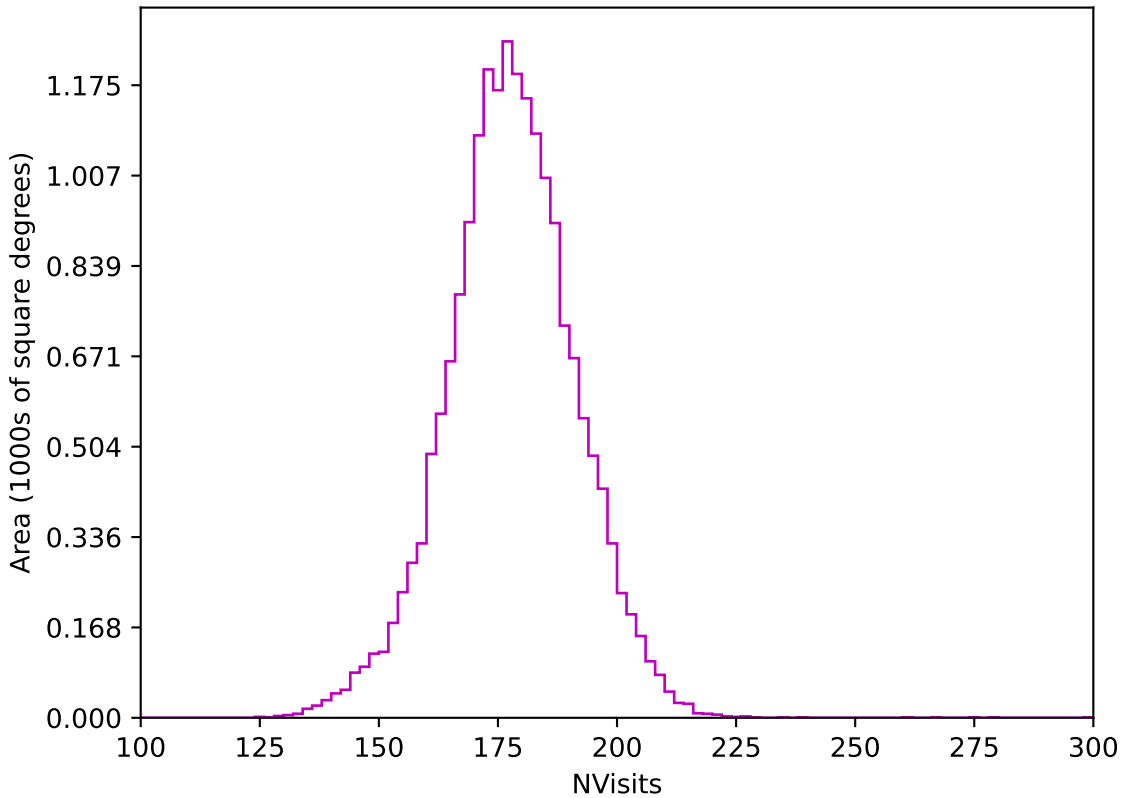
weather_cloudso4v3.4_10yrs WFD z band: NVisits
