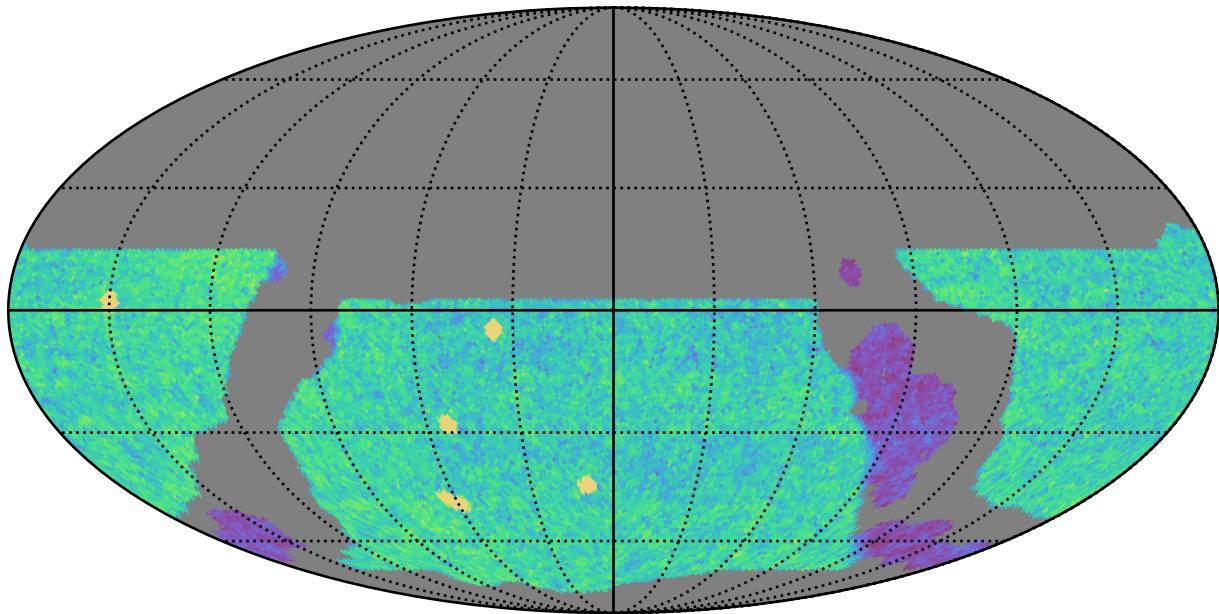
weather_cloudso4v3.4_10yrs WFD u band: NVisits
