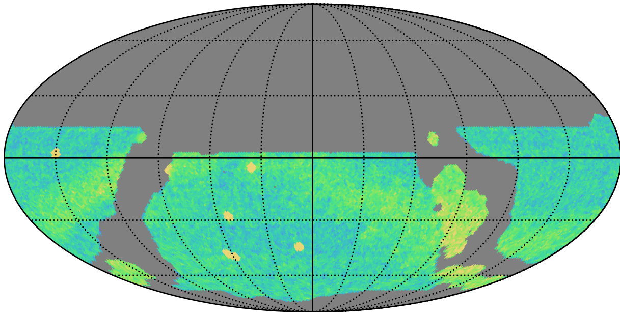
weather_cloudso4v3.4_10yrs WFD r band: NVisits
