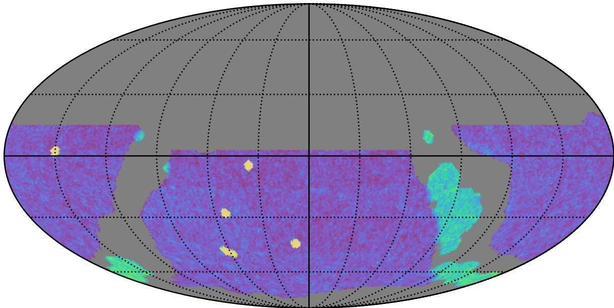
weather_cloudso4v3.4_10yrs WFD g band: NVisits
