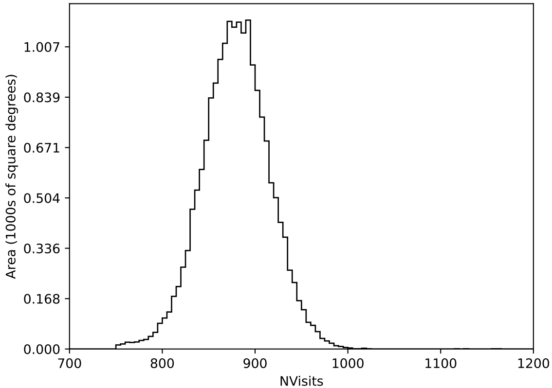
weather_cloudso4v3.4_10yrs WFD all bands: NVisits
