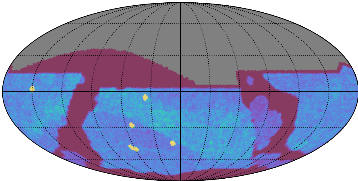
weather_cloudso4v3.4_10yrs All sky z band: NVisits
