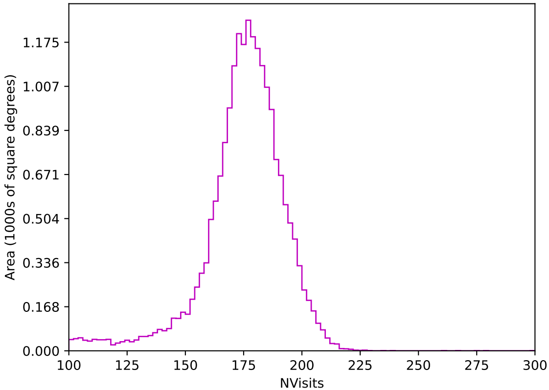
weather_cloudso4v3.4_10yrs All sky z band: NVisits
