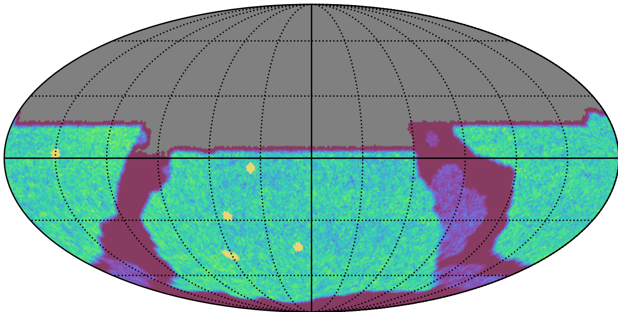
weather_cloudso4v3.4_10yrs All sky u band: NVisits
