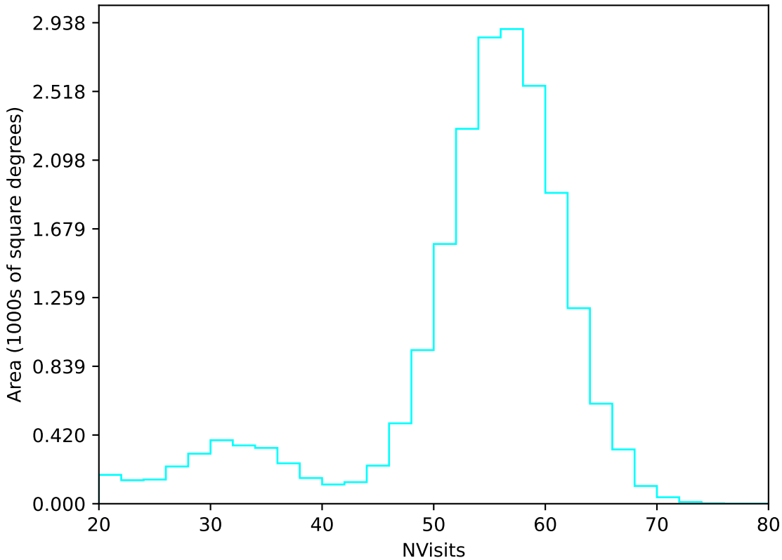
weather_cloudso4v3.4_10yrs All sky u band: NVisits
