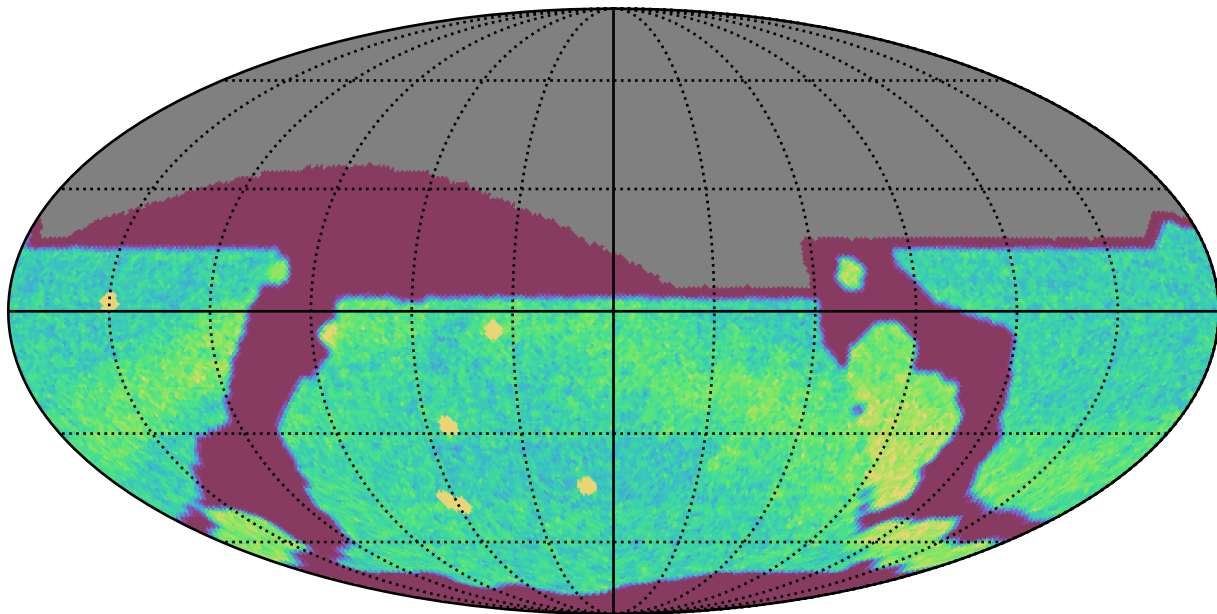
weather_cloudso4v3.4_10yrs All sky r band: NVisits
