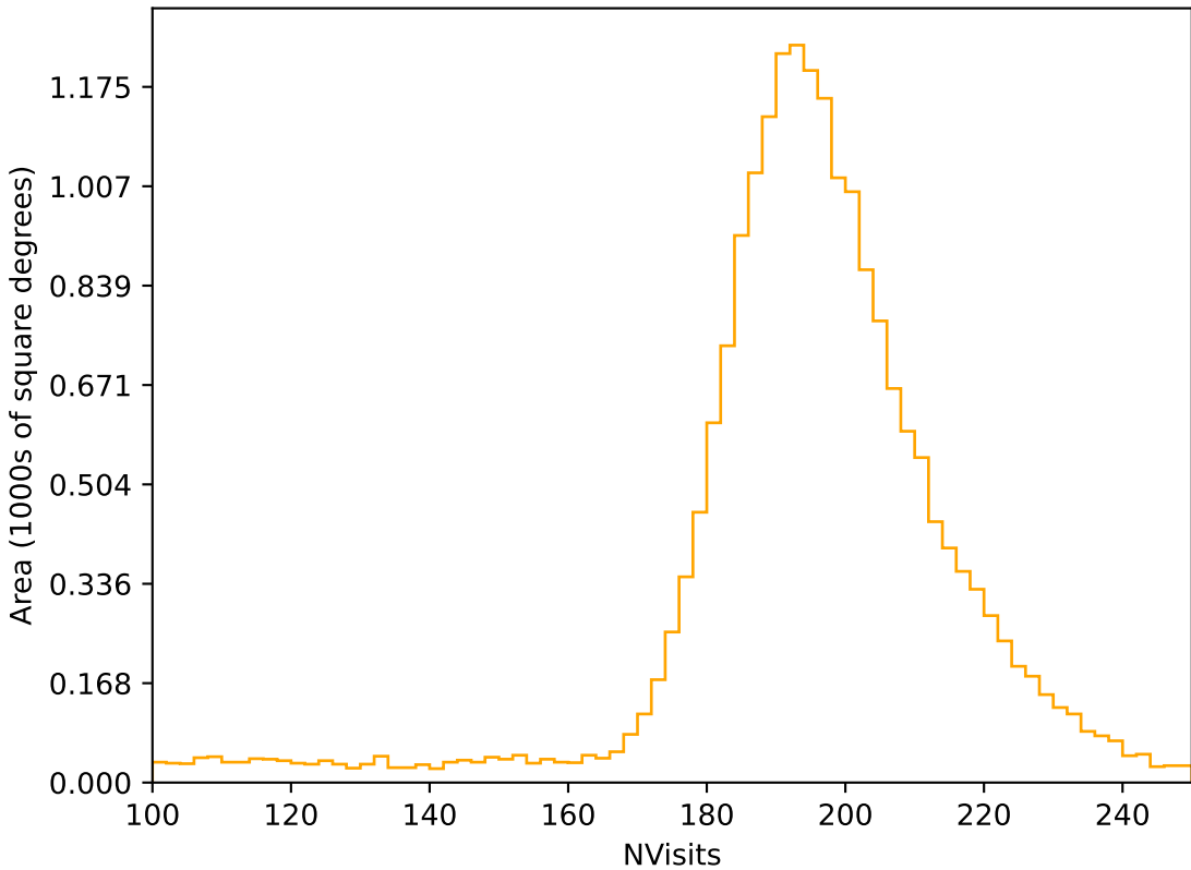
weather_cloudso4v3.4_10yrs All sky r band: NVisits
