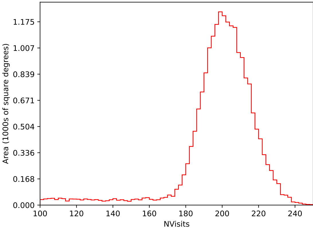
weather_cloudso4v3.4_10yrs All sky i band: NVisits
