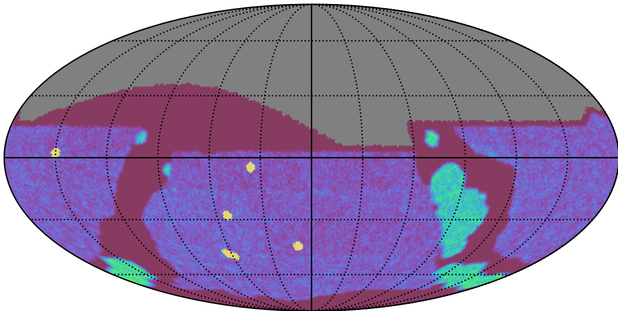
weather_cloudso4v3.4_10yrs All sky g band: NVisits
