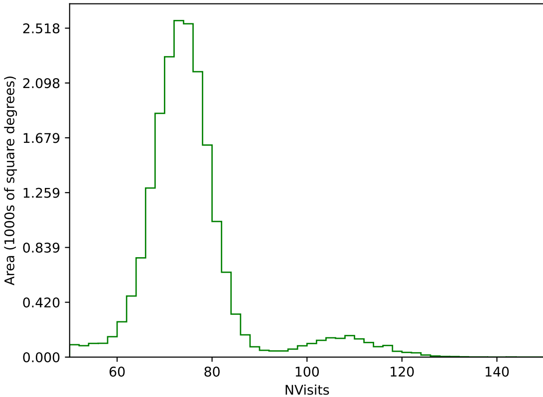
weather_cloudso4v3.4_10yrs All sky g band: NVisits
