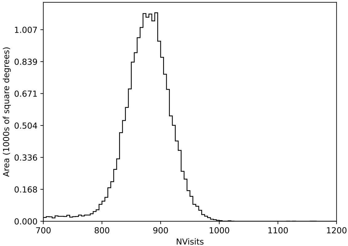
weather_cloudso4v3.4_10yrs All sky all bands: NVisits
