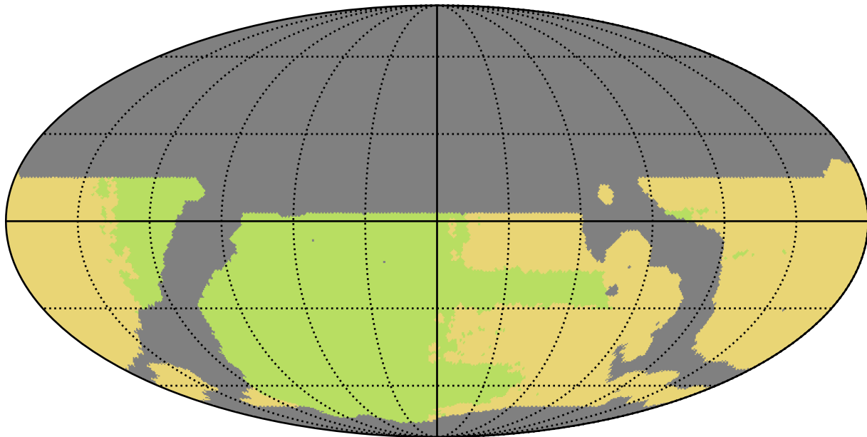
weather_cloudso4v3.4_10yrs WFD all bands: NSeasons
