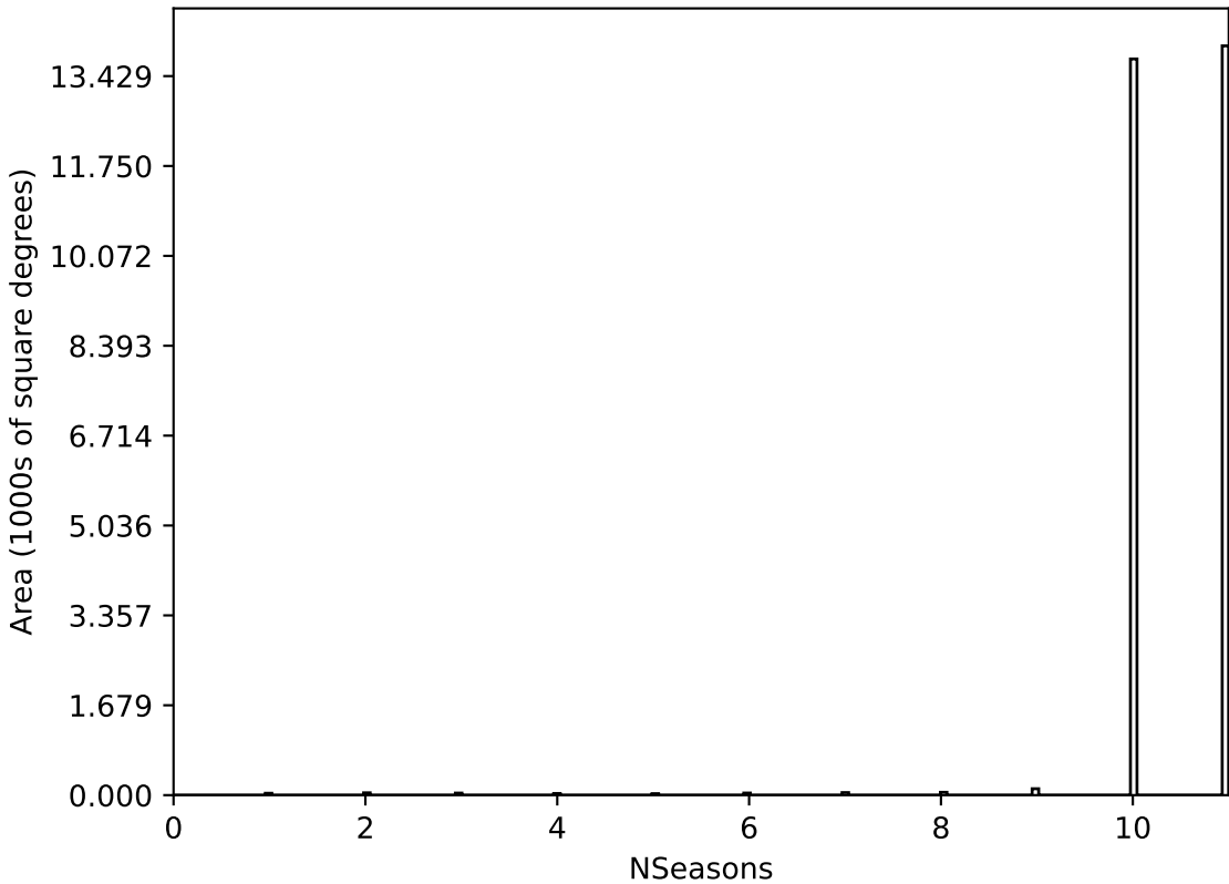
weather_cloudso4v3.4_10yrs All sky all bands: NSeasons
