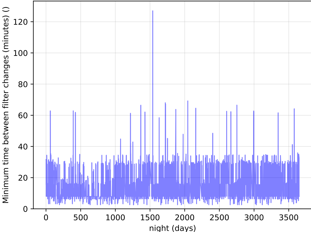
weather_cloudso4v3.4_10yrs Per Night: Minimum time between filter changes (minutes)
