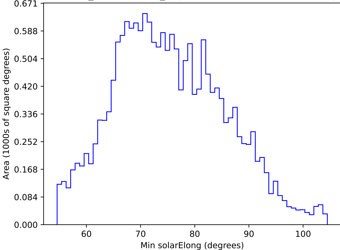
weather_cloudso4v3.4_10yrs WFD u band: Min solarElong
