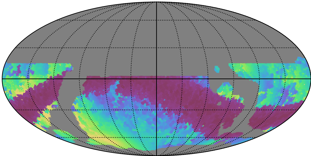
weather_cloudso4v3.4_10yrs WFD r band: Min solarElong
