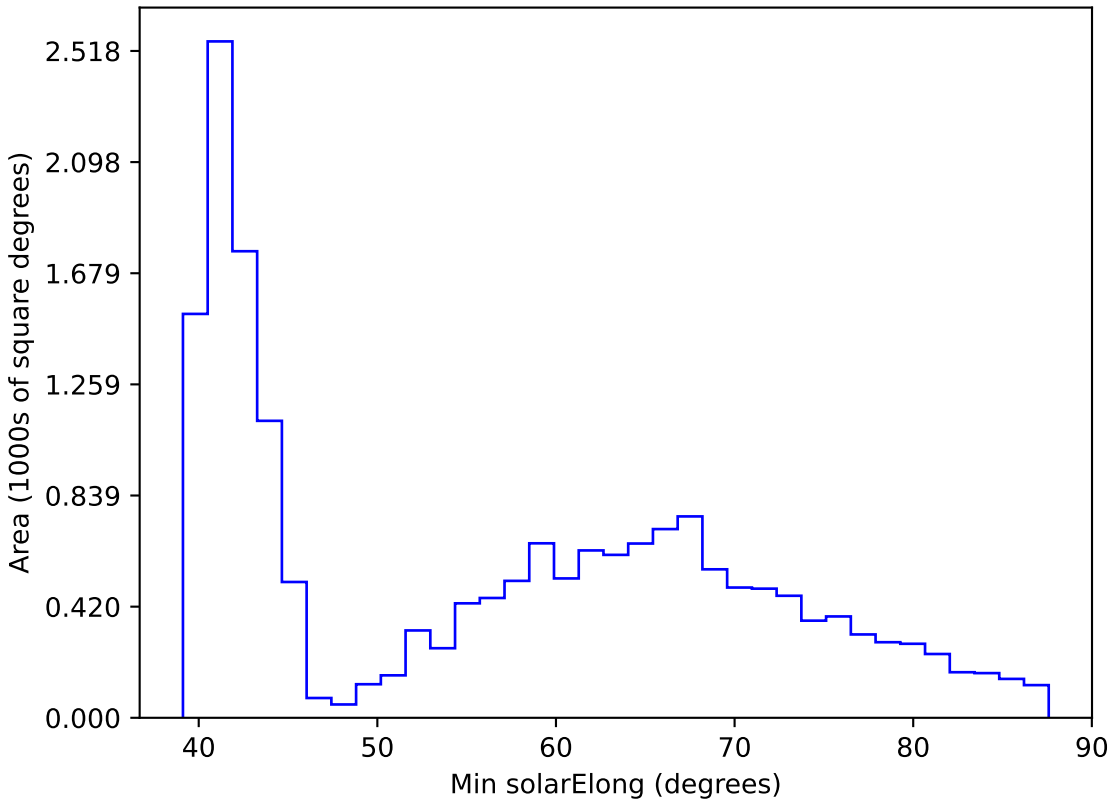
weather_cloudso4v3.4_10yrs WFD r band: Min solarElong
