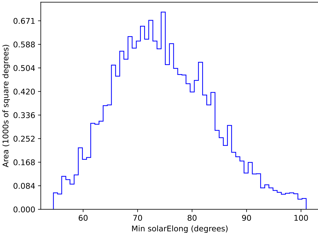
weather_cloudso4v3.4_10yrs WFD g band: Min solarElong
