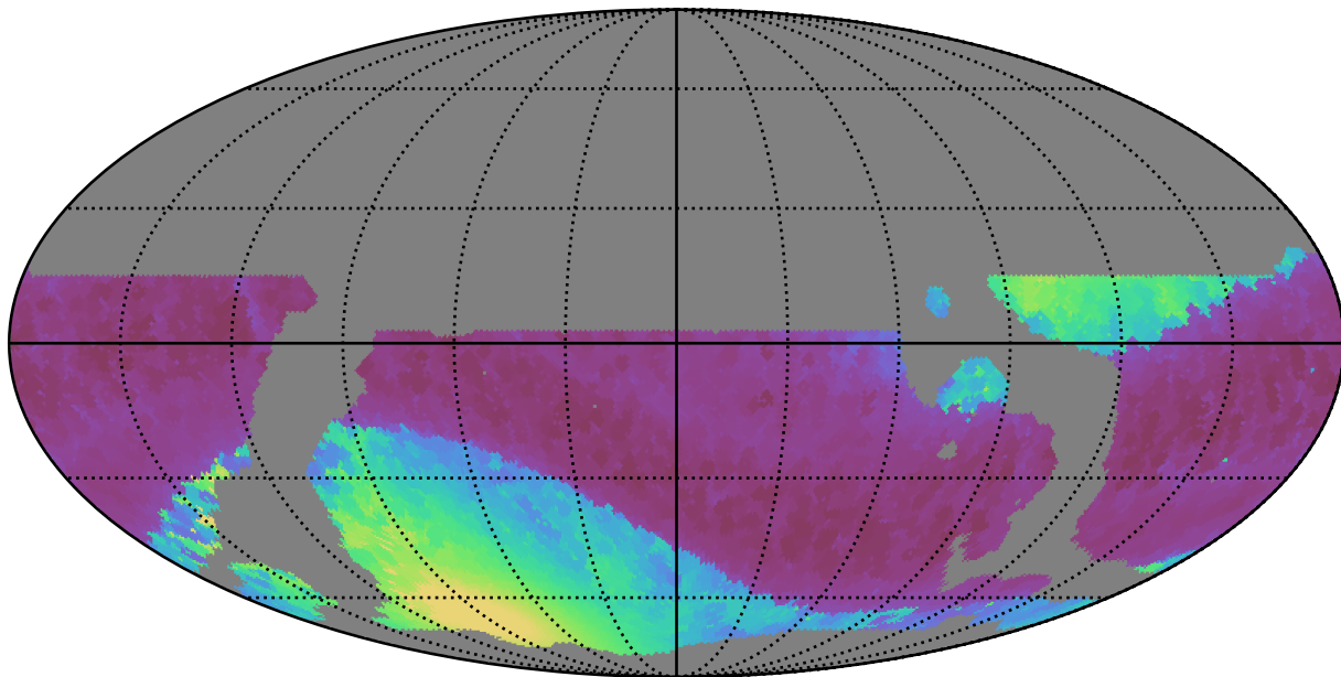
weather_cloudso4v3.4_10yrs WFD all bands: Min solarElong
