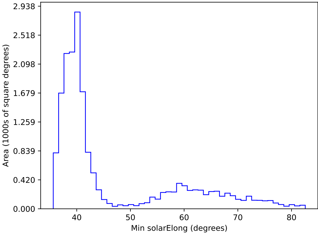
weather_cloudso4v3.4_10yrs WFD all bands: Min solarElong
