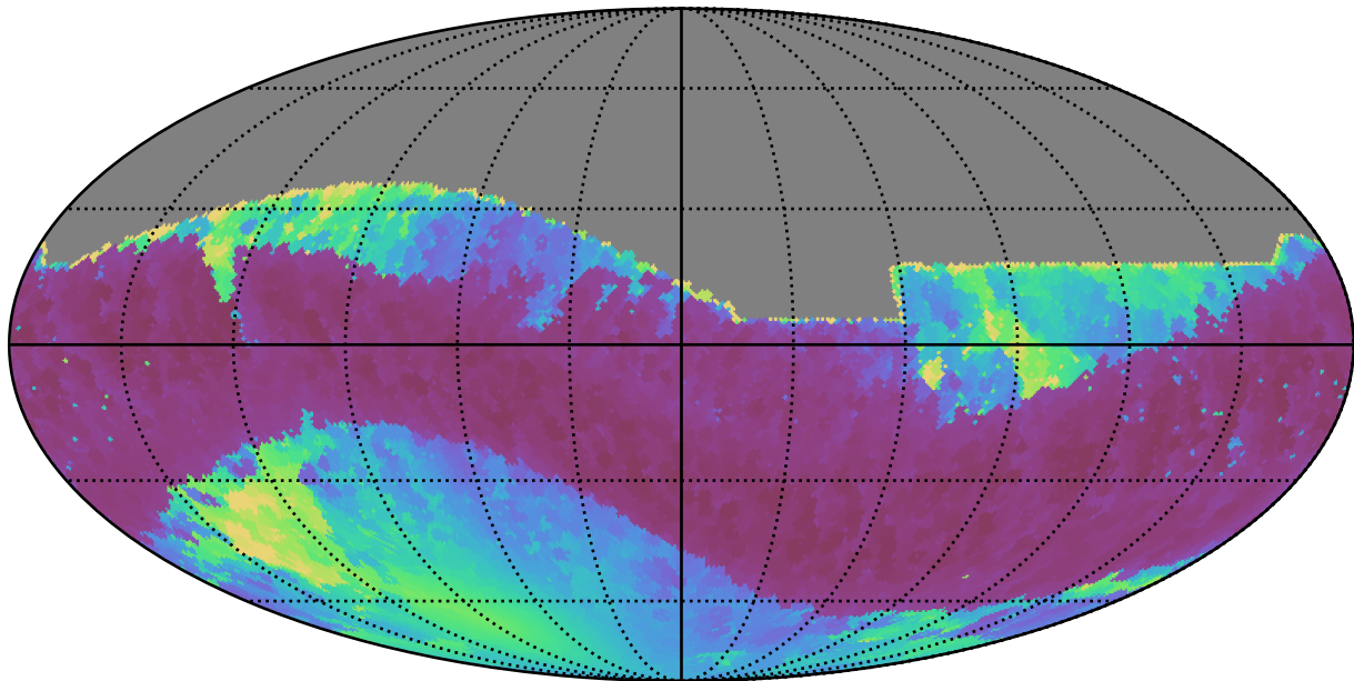
weather_cloudso4v3.4_10yrs All sky z band: Min solarElong
