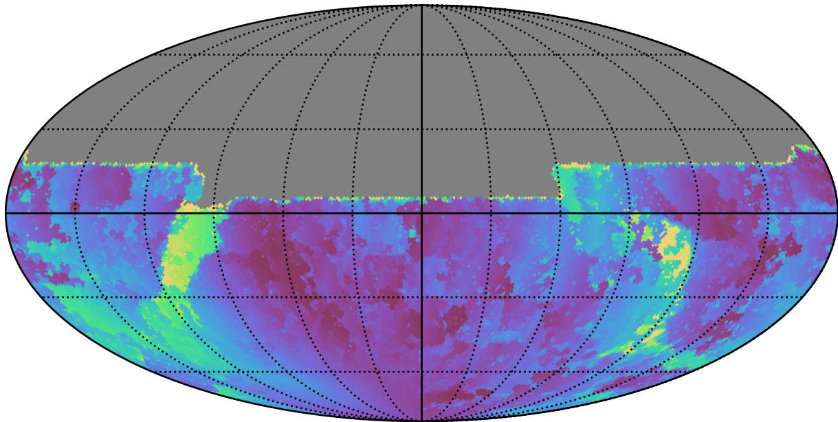
weather_cloudso4v3.4_10yrs All sky u band: Min solarElong
