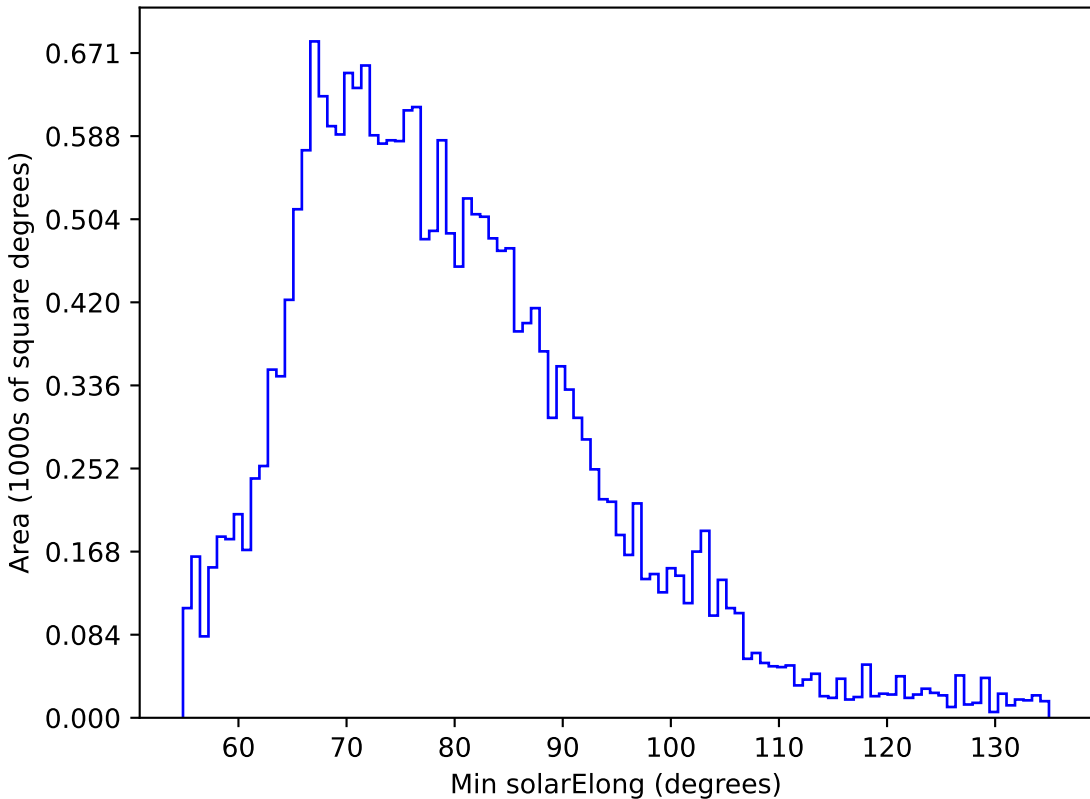
weather_cloudso4v3.4_10yrs All sky u band: Min solarElong
