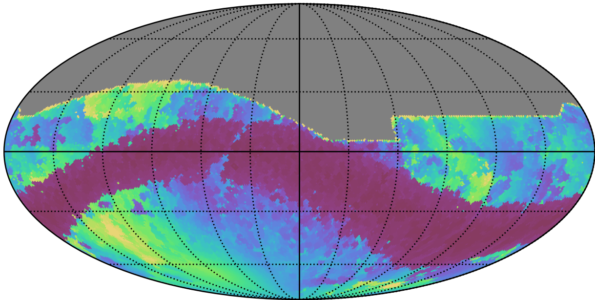
weather_cloudso4v3.4_10yrs All sky r band: Min solarElong
