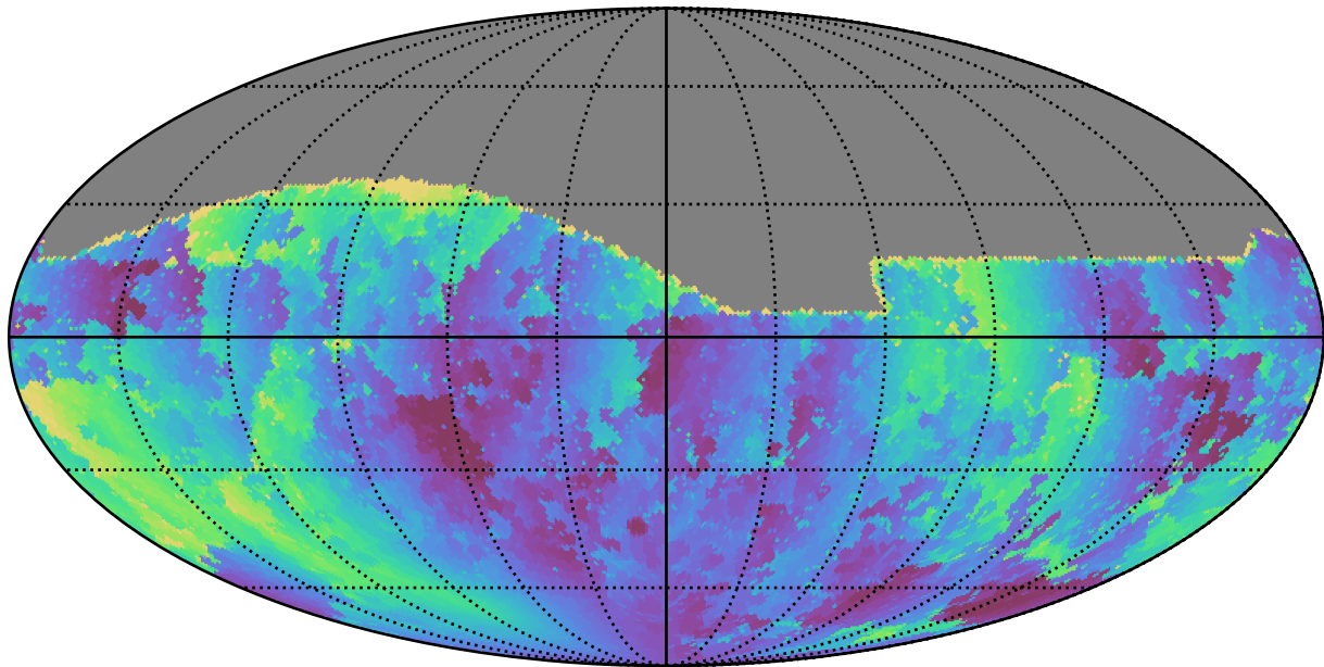
weather_cloudso4v3.4_10yrs All sky g band: Min solarElong
