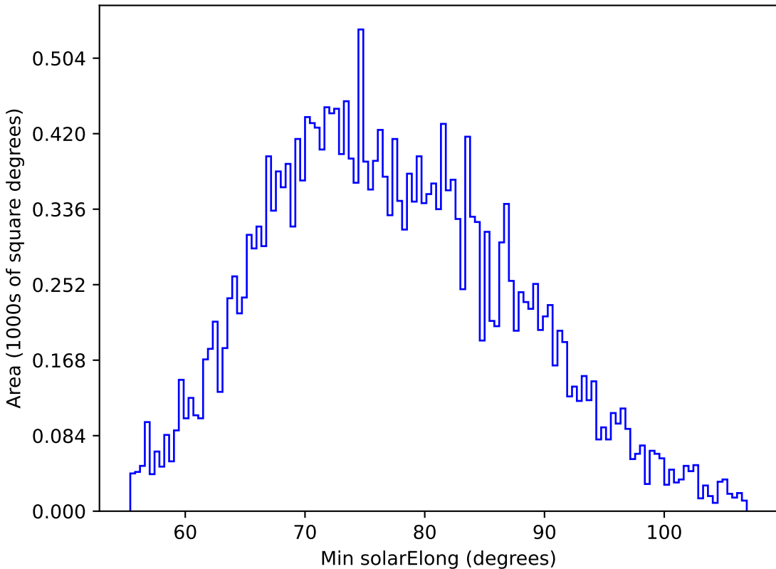
weather_cloudso4v3.4_10yrs All sky g band: Min solarElong
