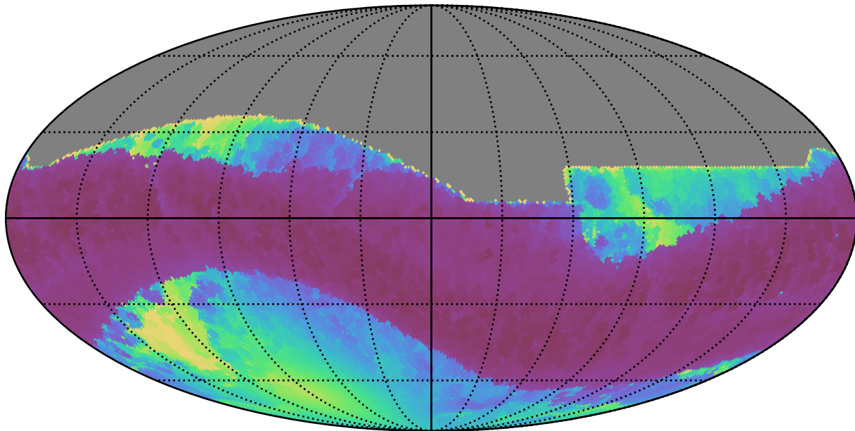
weather_cloudso4v3.4_10yrs All sky all bands: Min solarElong
