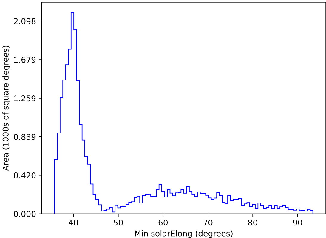
weather_cloudso4v3.4_10yrs All sky all bands: Min solarElong
