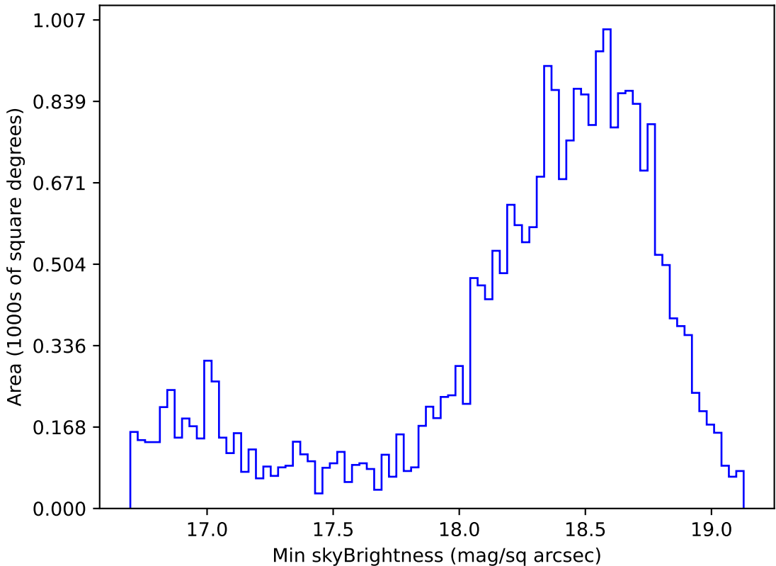
weather_cloudso4v3.4_10yrs Yr 1 z band: Min skyBrightness
