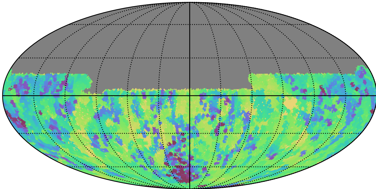
weather_cloudso4v3.4_10yrs Yr 1 y band: Min skyBrightness
