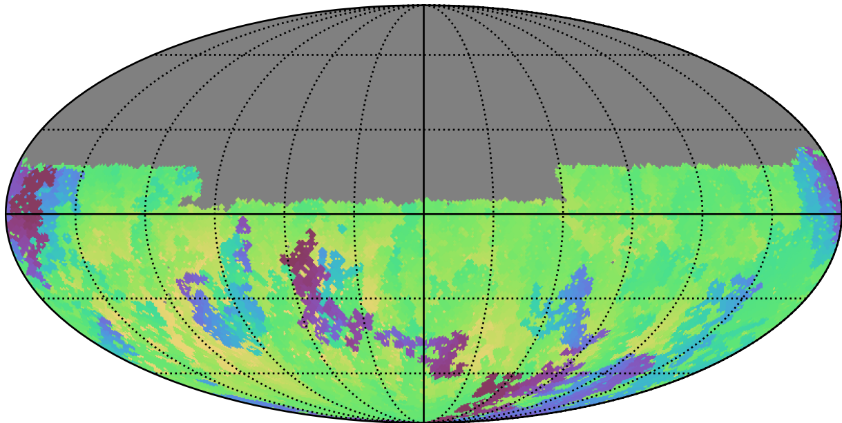
weather_cloudso4v3.4_10yrs Yr 1 u band: Min skyBrightness
