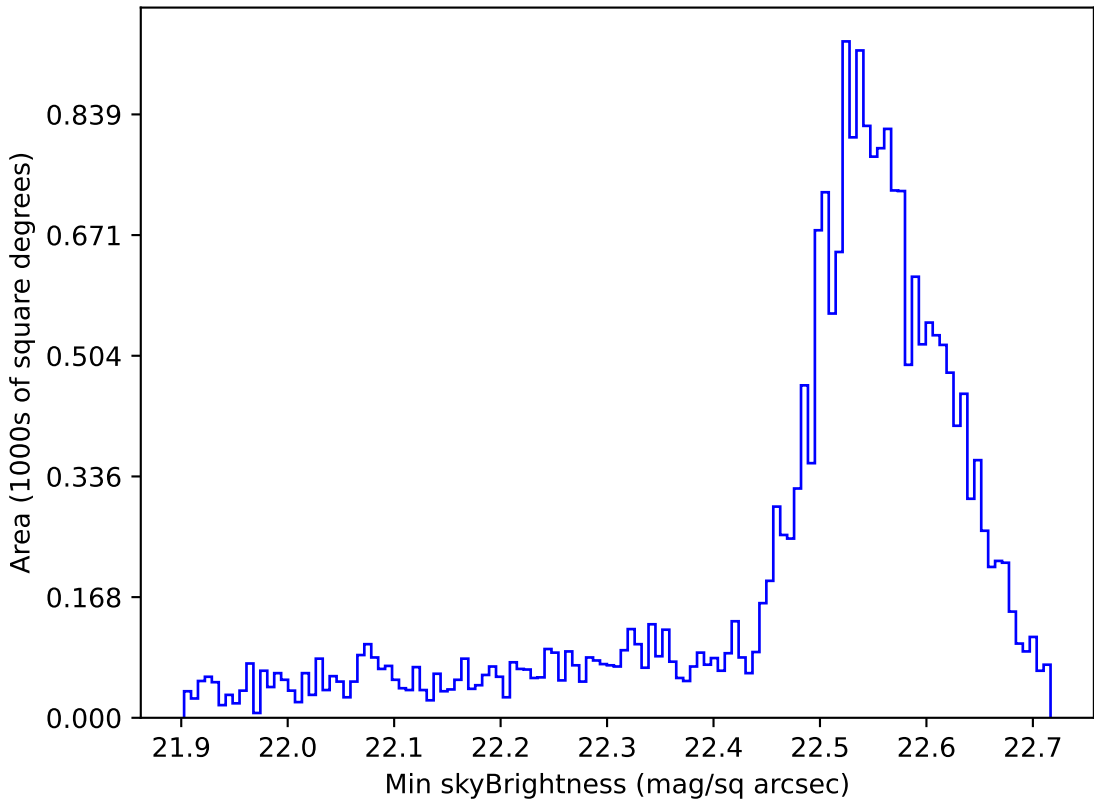
weather_cloudso4v3.4_10yrs Yr 1 u band: Min skyBrightness
