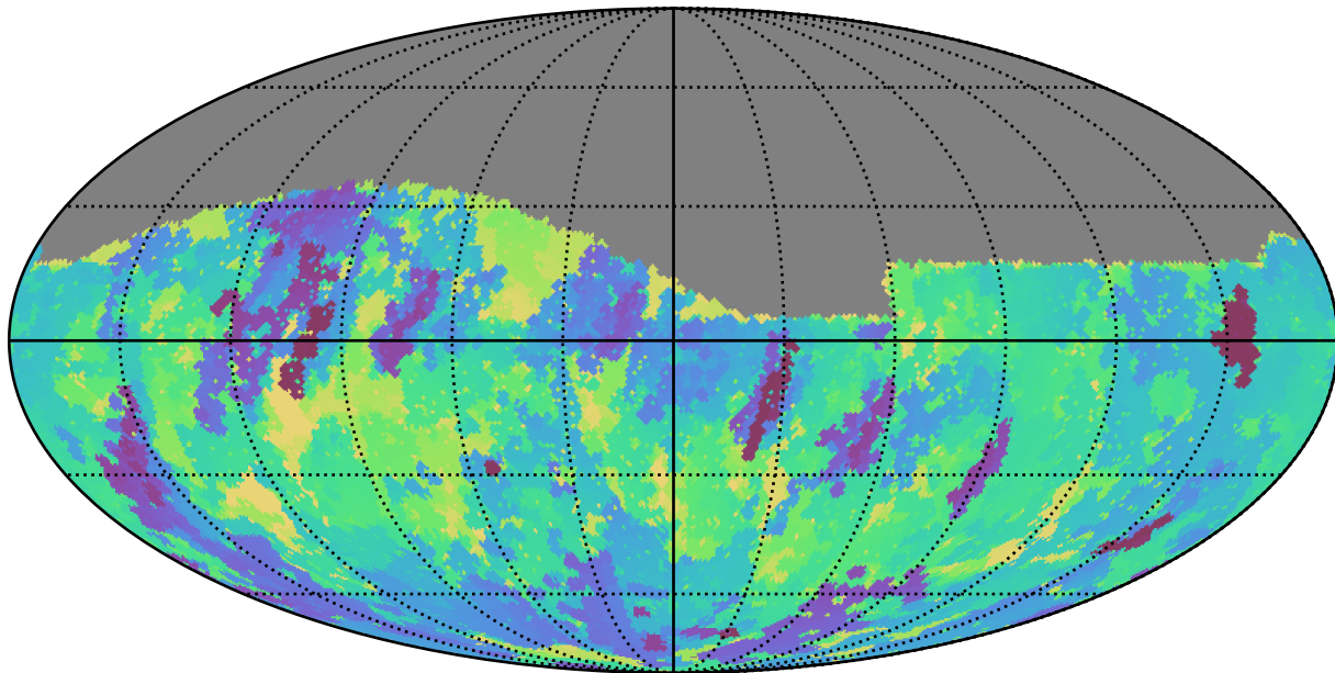
weather_cloudso4v3.4_10yrs Yr 1 r band: Min skyBrightness
