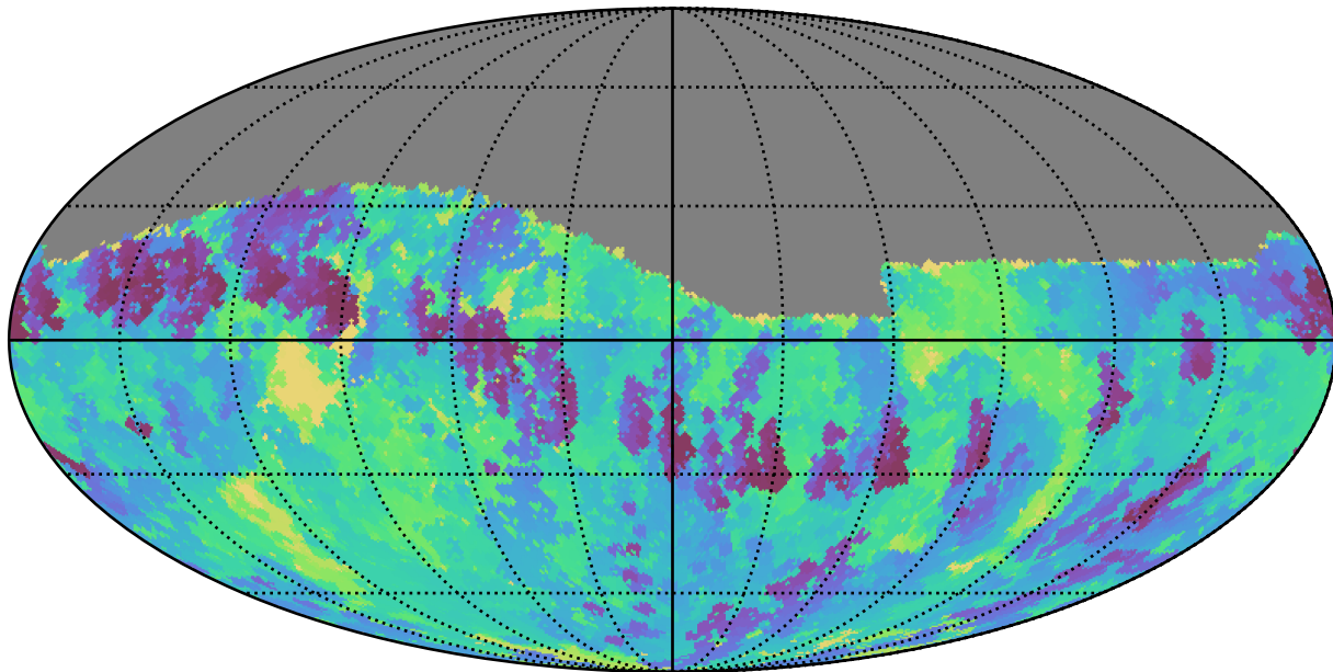
weather_cloudso4v3.4_10yrs Yr 1 i band: Min skyBrightness
