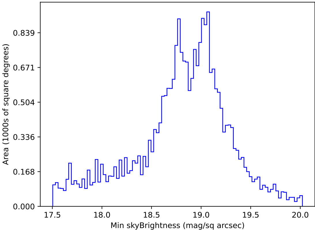
weather_cloudso4v3.4_10yrs Yr 1 i band: Min skyBrightness
