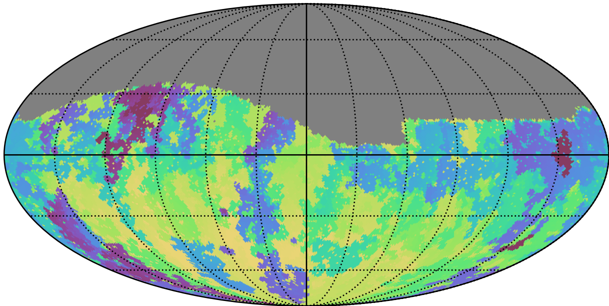
weather_cloudso4v3.4_10yrs Yr 1 g band: Min skyBrightness
