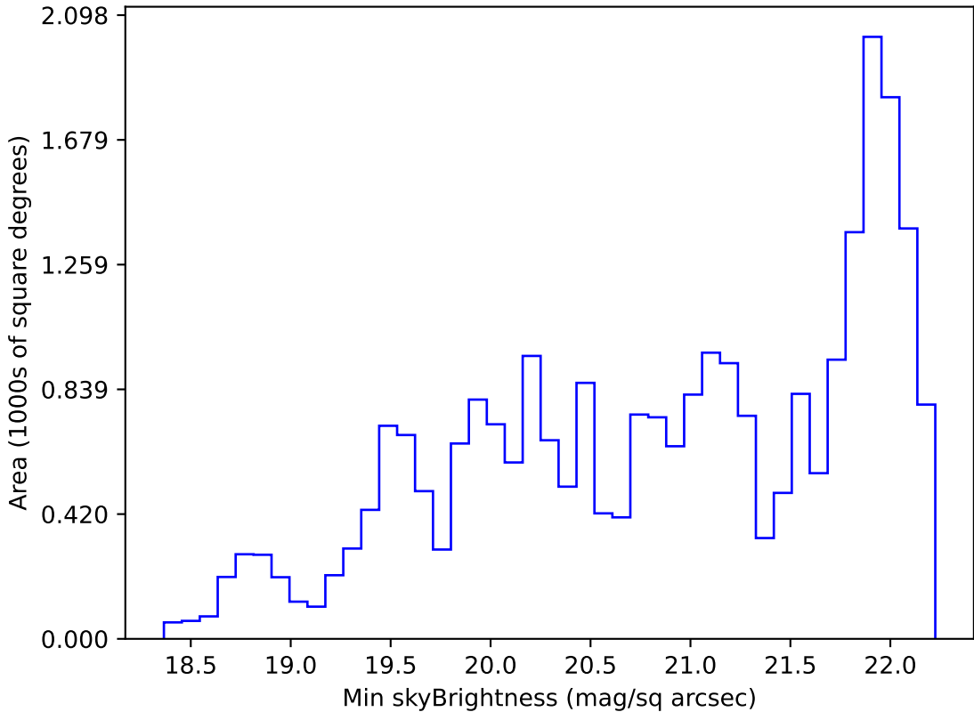
weather_cloudso4v3.4_10yrs Yr 1 g band: Min skyBrightness
