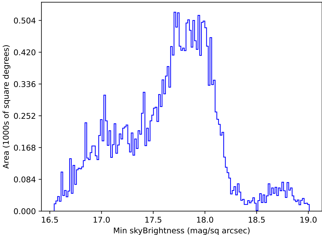
weather_cloudso4v3.4_10yrs Yr 1 all bands: Min skyBrightness
