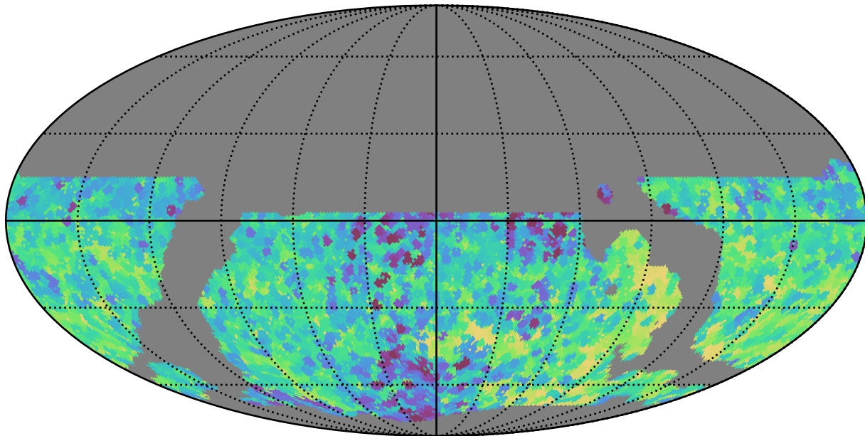
weather_cloudso4v3.4_10yrs WFD y band: Min skyBrightness
