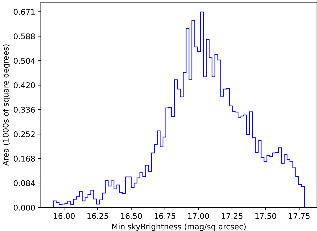
weather_cloudso4v3.4_10yrs WFD y band: Min skyBrightness
