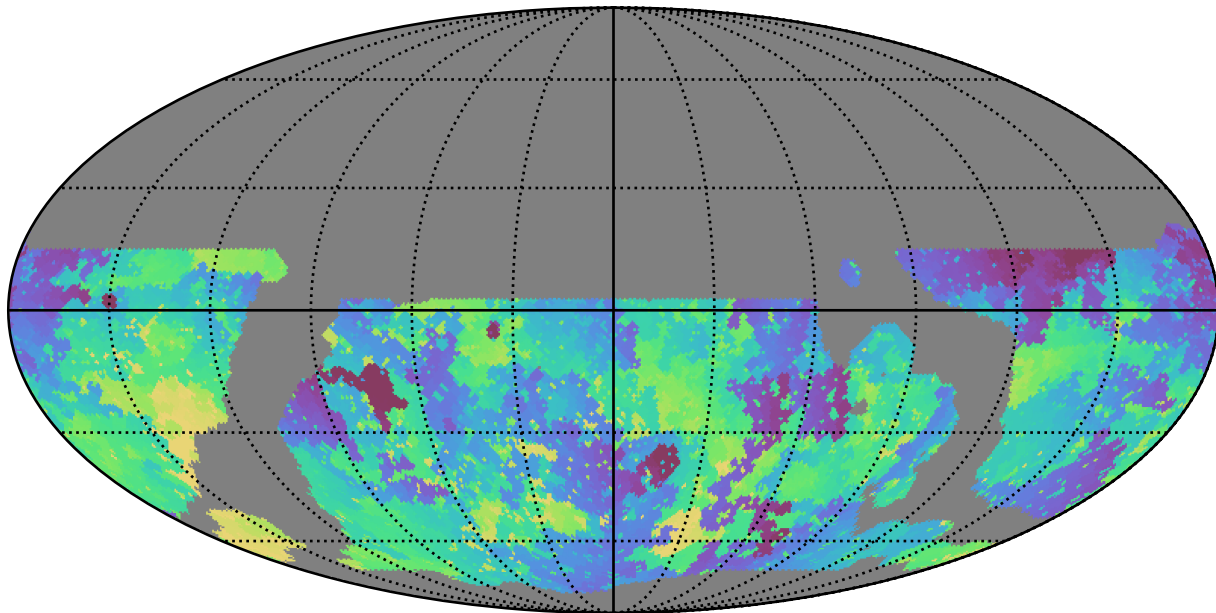
weather_cloudso4v3.4_10yrs WFD u band: Min skyBrightness
