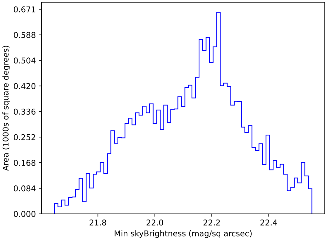
weather_cloudso4v3.4_10yrs WFD u band: Min skyBrightness
